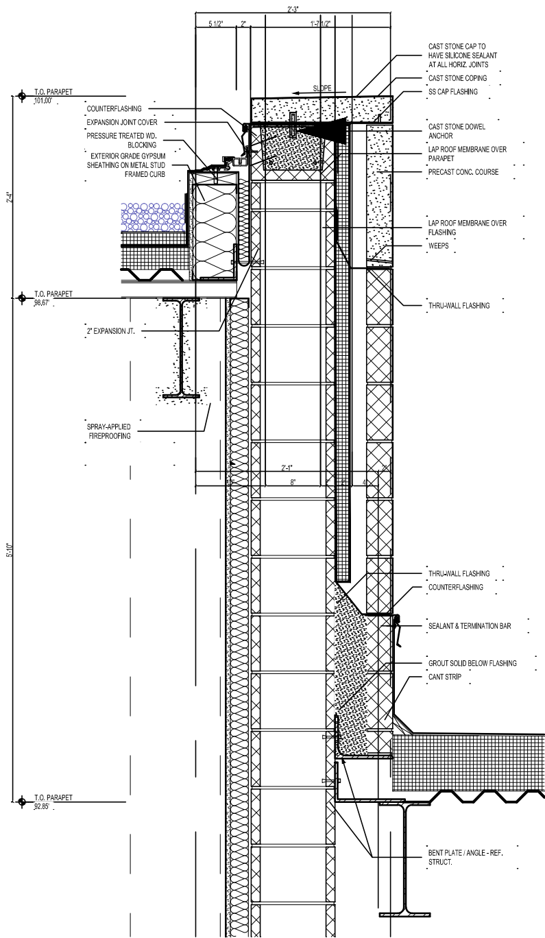
Roof Parapet Brick & Precast
