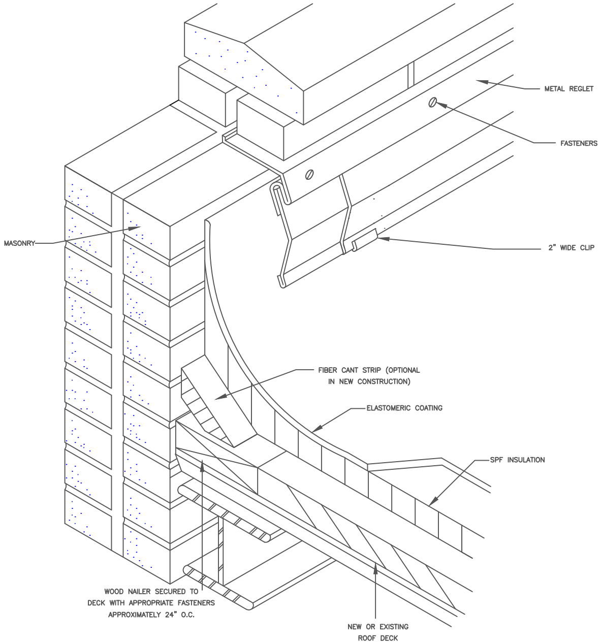
Parapet Roof Detail 3
