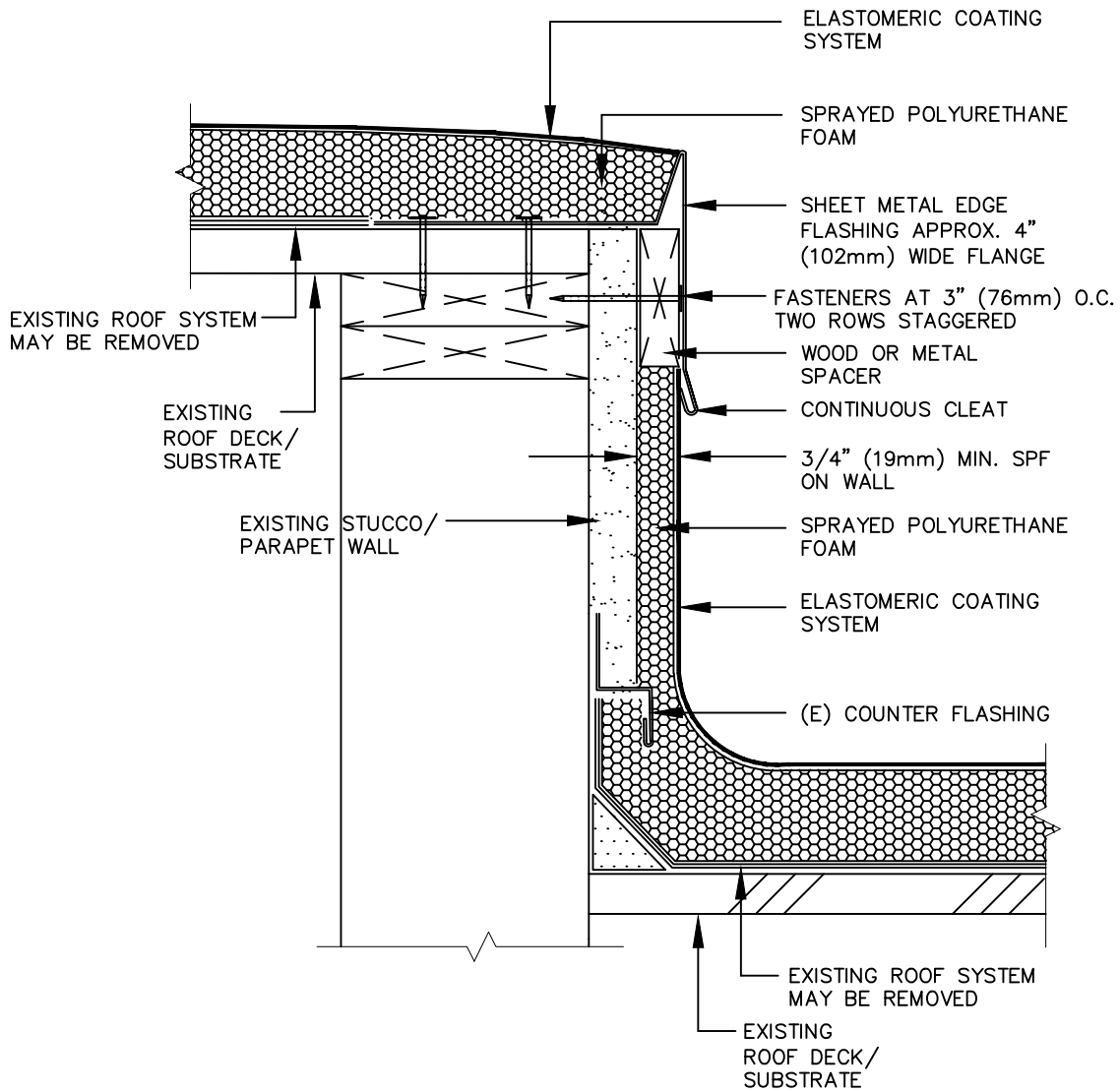
Roof_Transition_Wall[1]
