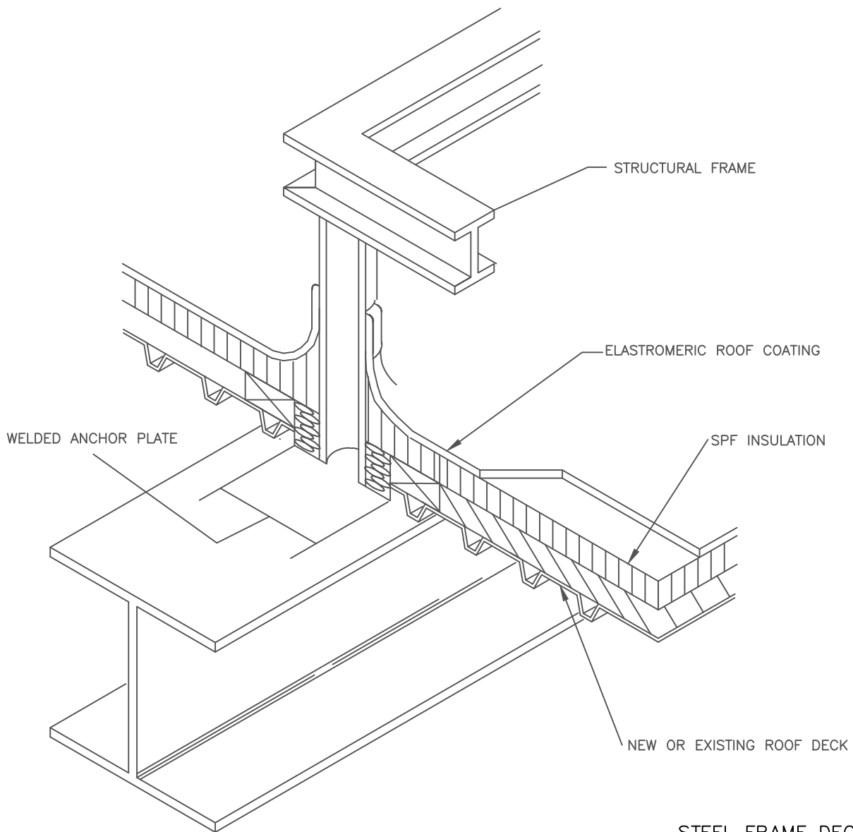
STEEL FRAME DECK DTL
